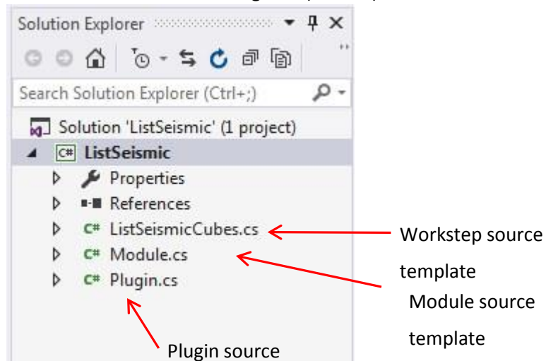
Figure 11: Example Project Source Files in Solution Explorer
