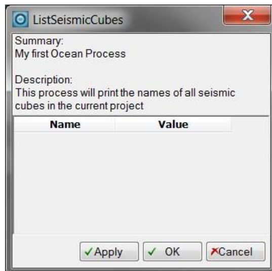
Figure 13: ListSeismicCubes Dialog
