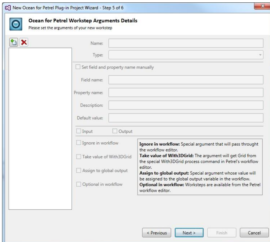
Figure 9: Ocean Workstep Argument Details
